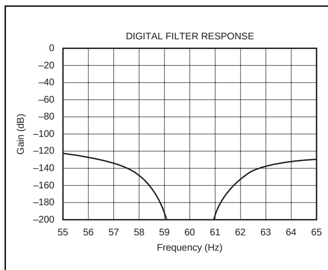
FIGURE 11. Expanded Digital Filter Response (60Hz with a 10Hz Notch).
