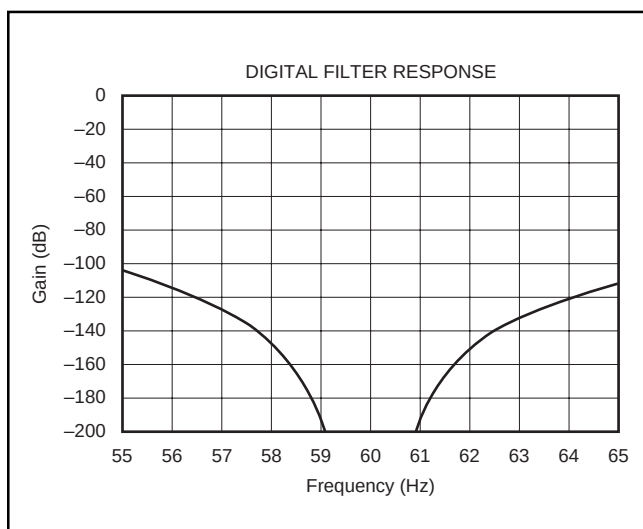
FIGURE 10. Expanded Digital Filter Response (60Hz with a 60Hz Notch).
