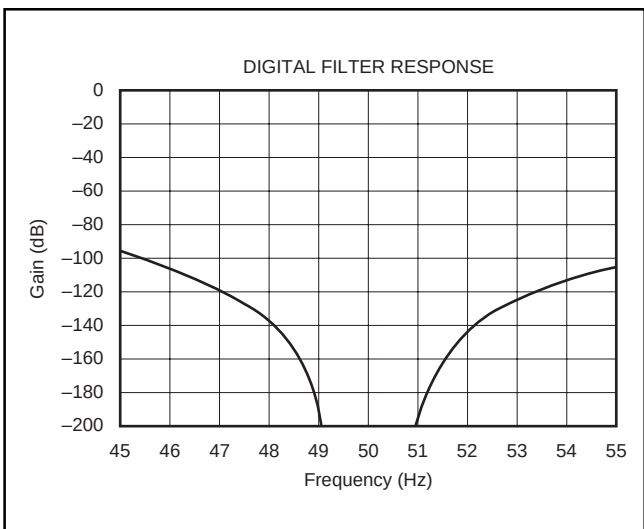
FIGURE 8. Expanded Digital Filter Response (50Hz with a 50Hz Notch).
