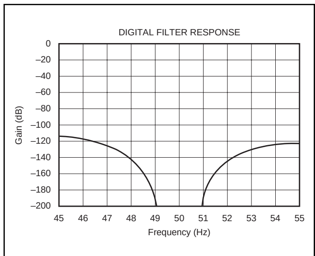
FIGURE 9. Expanded Digital Filter Response (50Hz with a 10Hz Notch).
