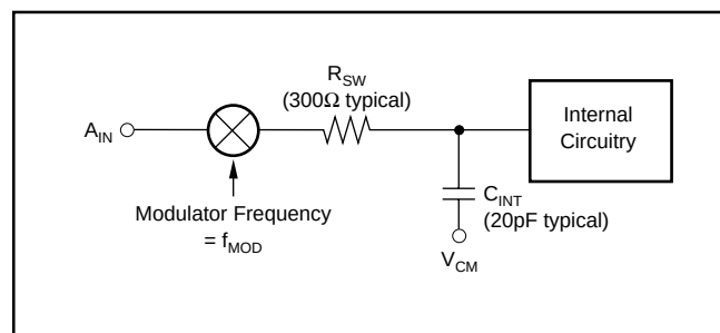
FIGURE 1. Analog-Input Structure.
