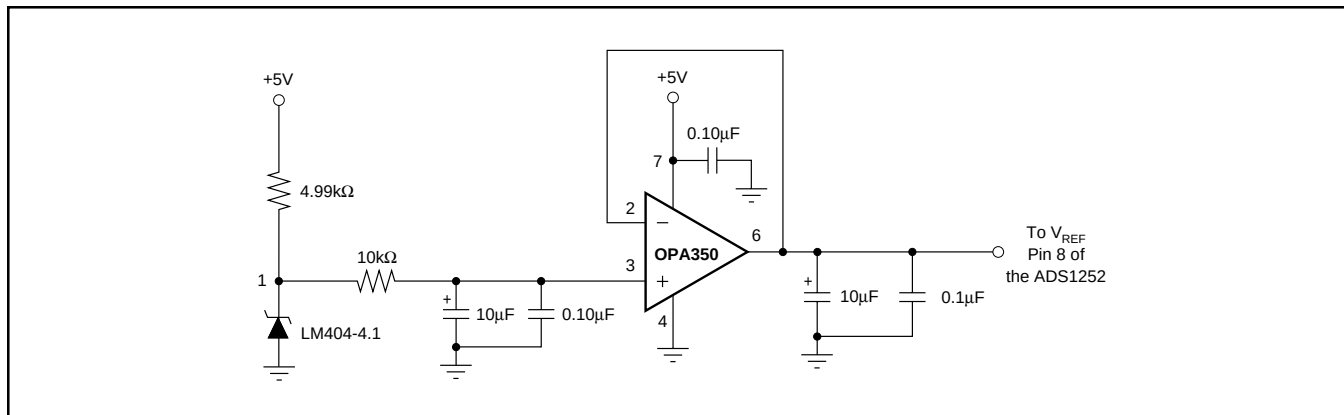
FIGURE 3. Recommended External Voltage Reference Circuit for Best Low-Noise Operation with the ADS1252.
